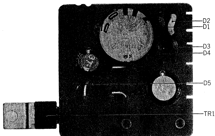
FIG. 12 PHOTO OF POWER SUPPLY P.C. BOARD (MU-5017)
