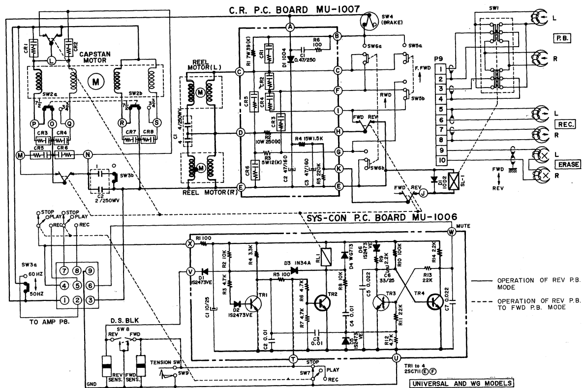
SCHEMATIC 3
