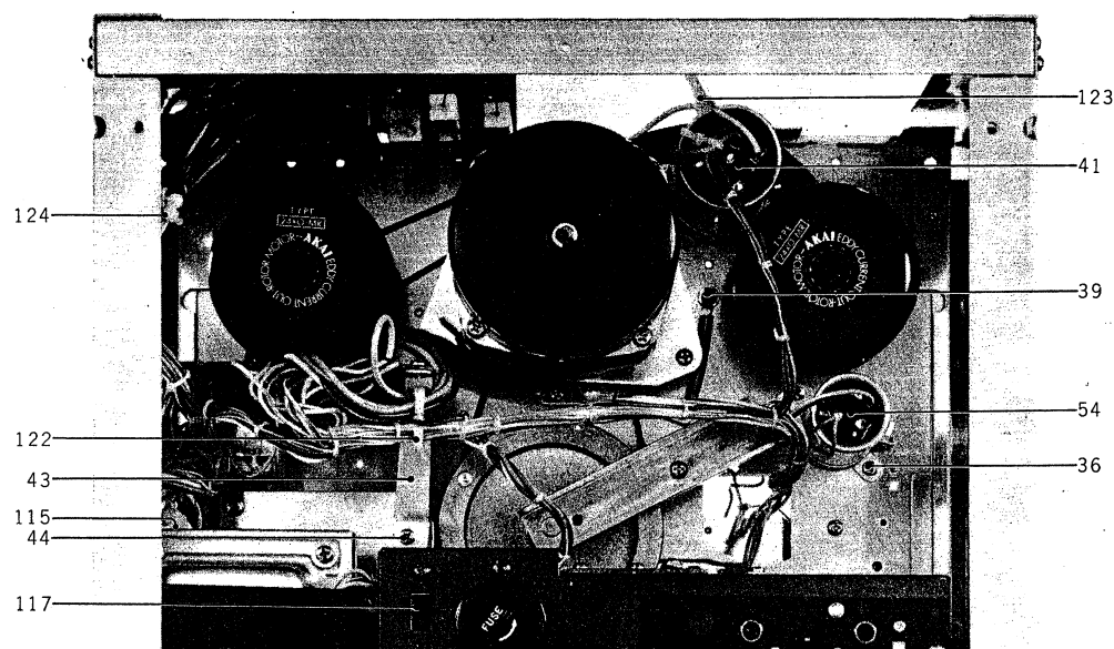
FIG. 6 (B) PHOTO OF MECHANISM ASSEMBLY BLOCK
