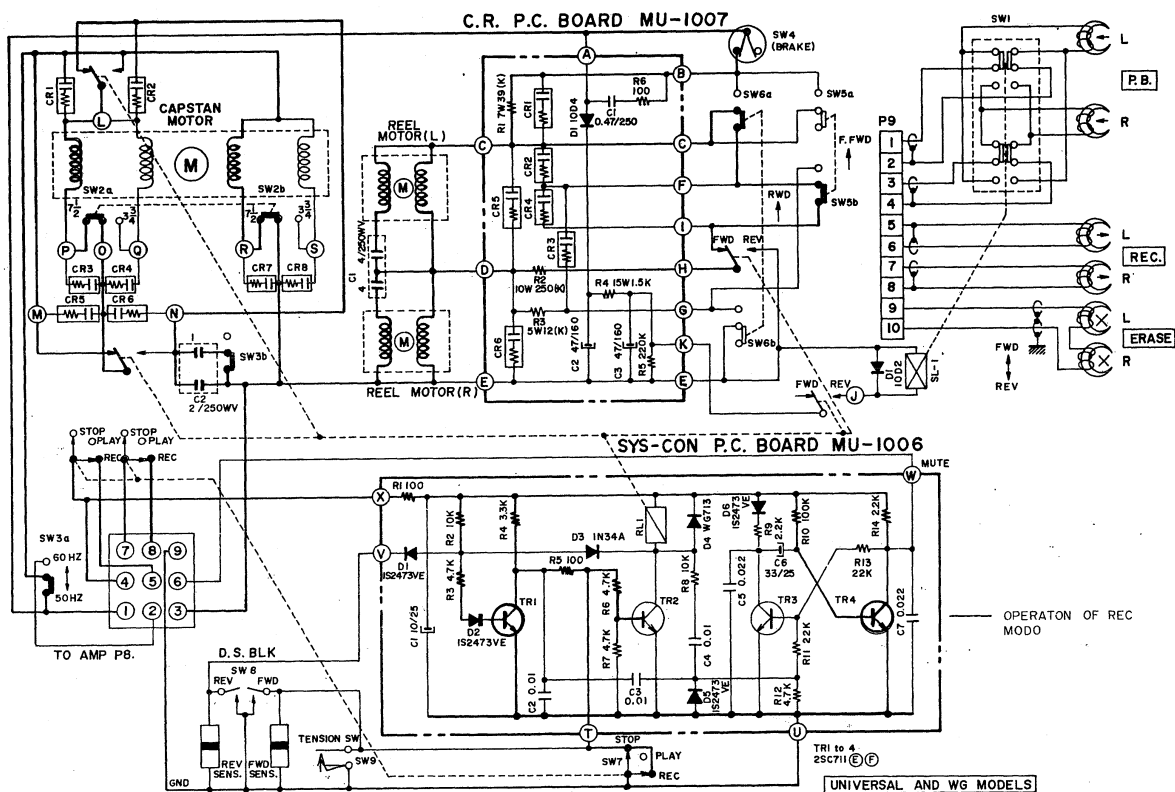
SCHEMATIC 4
