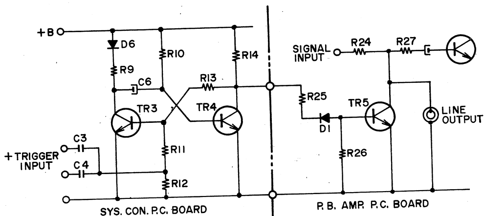
SCHEMATIC 7
