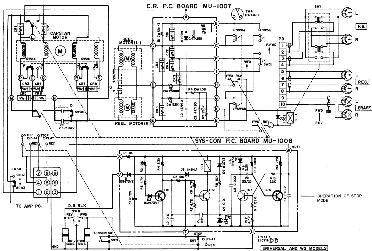
SCHEMATIC 1
