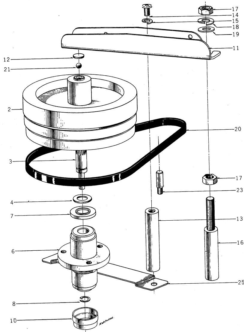
FIG. 4 ILLUSTRATION OF FLYWHEEL BLOCK
