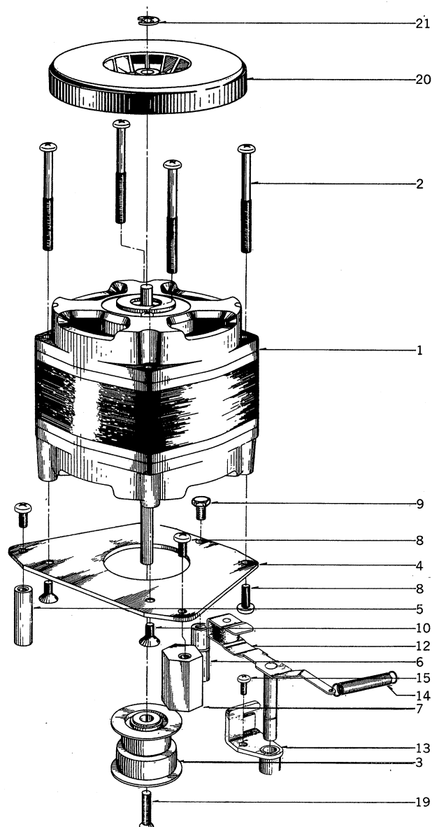
FIG. 3 ILLUSTRATION OF MAIN MOTOR BLOCK
