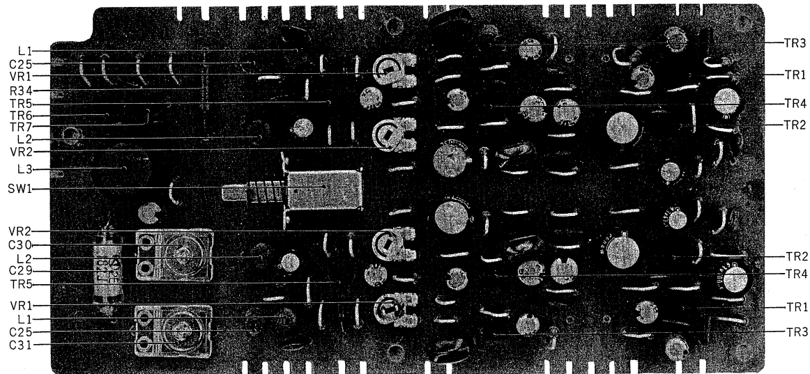
FIG. 9 PHOTO OF REC. AMP. P.C. BOARD (MU-5016)
