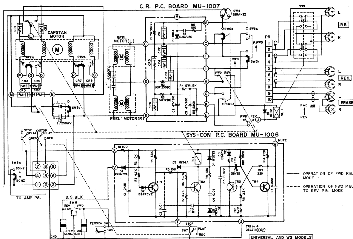
SCHEMATIC 2
