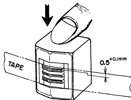
LELT CH. P.B. LEVEL ADJUSTMENT
