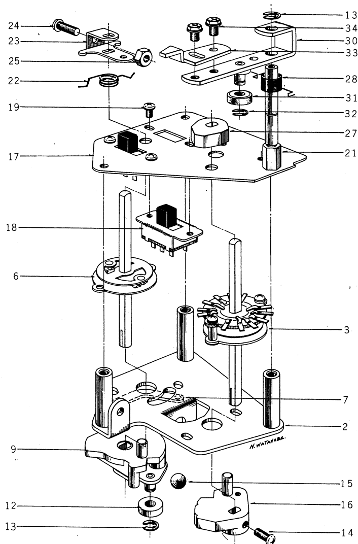
FIG. 5 ILLUSTRATION OF SWITCH BLOCK
