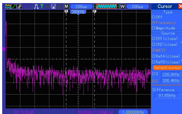
Frequency Cursors
