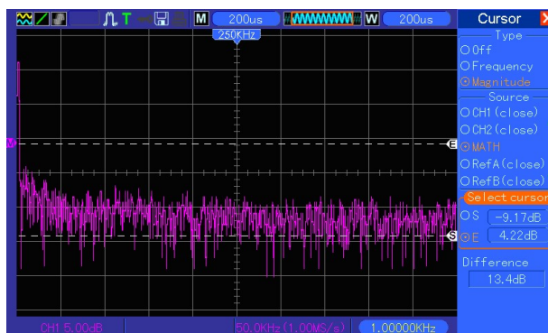
Amplitude Cursors
